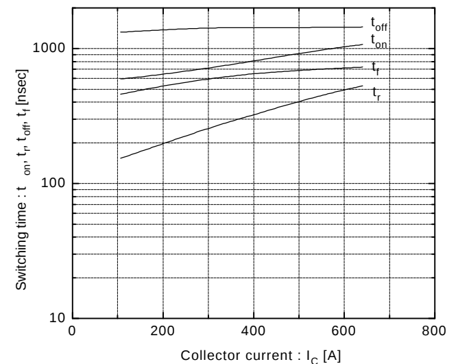
Switching time vs. Collector current V_{CC} = 600V, R_G = 1.8\Omega, V_{GE} = \pm 15V, T_J = 125^\circ\text{C}
