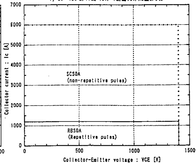
Reverse biased safty operating area T_j=25\sim 125^\circ C , +V_{GE}=15V , -V_{GE}\leq 15V , R_G\geq 2.0\Omega
