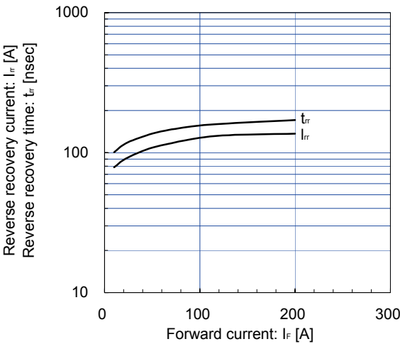
Reverse Recovery Characteristics (typ.) V_{CC}=600\text{V} , V_{GE}=\pm 15\text{V} , R_G=1.6\Omega , T_J=125^\circ\text{C}
