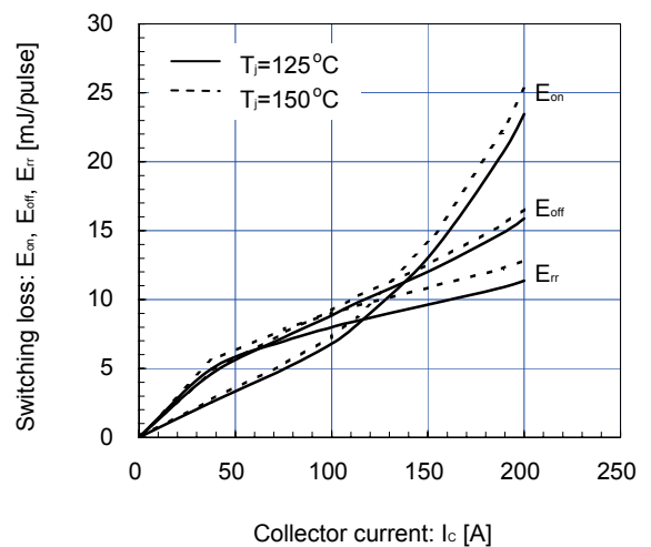
Switching loss vs. Collector current (typ.) V_{CC}=600V , V_{GE}=\pm 15V , R_G=1.6\Omega , T_J=125, 150^\circ C
