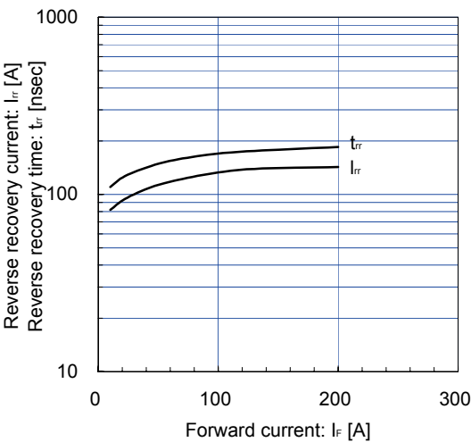
Reverse Recovery Characteristics (typ.) V_{CC}=600\text{V} , V_{GE}=\pm 15\text{V} , R_G=1.6\Omega , T_J=150^\circ\text{C}
