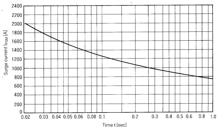
Surge Current
