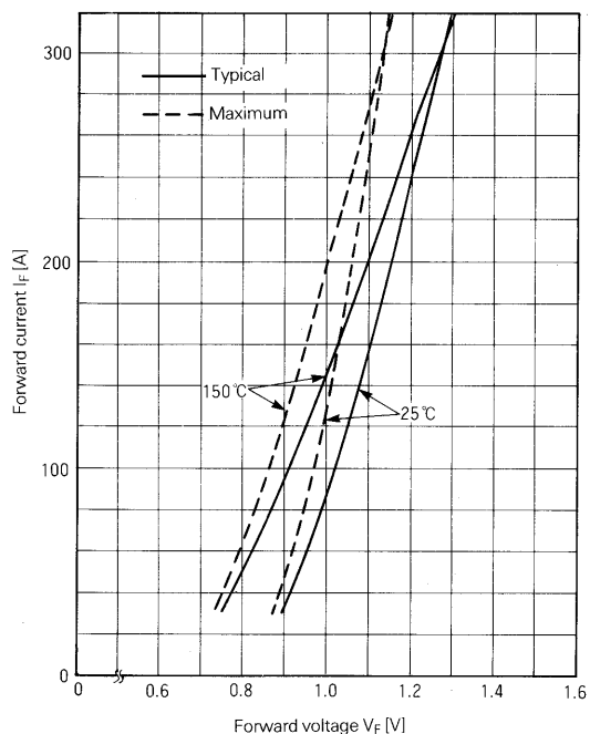
Forward Characteristics
