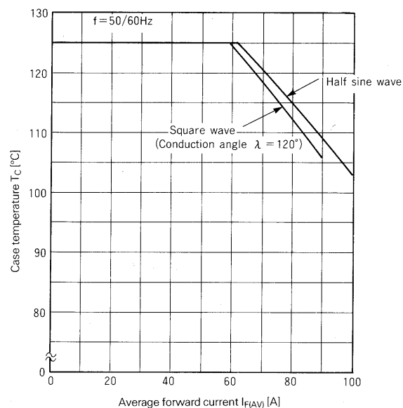
Case Temperature — Forward Average Current
