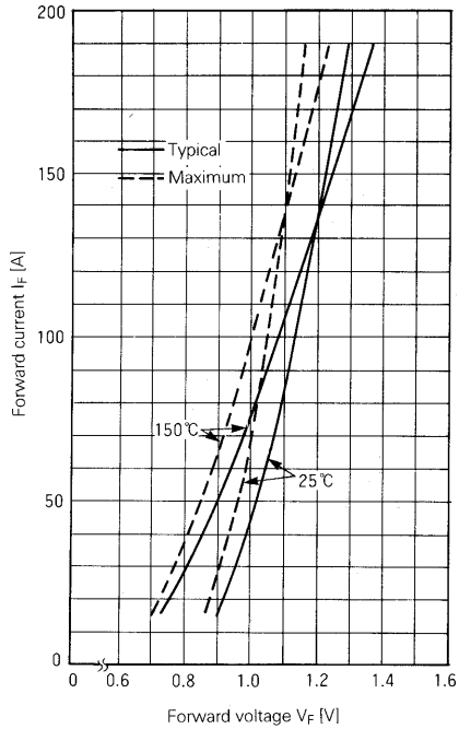
Forward Characteristics
