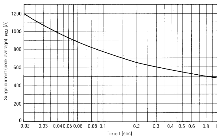
Surge Current
