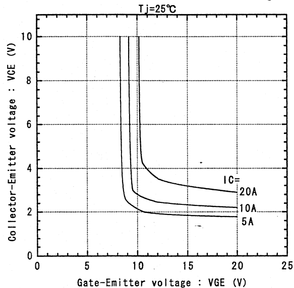
Collector-Emitter vs. Gate-Emitter voltage
