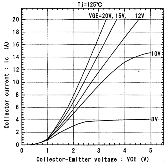
Collector-Emitter voltage vs. Collector current
