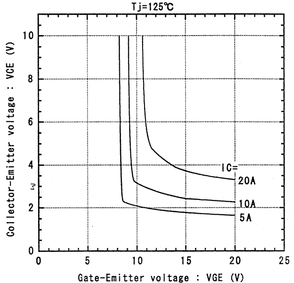
Collector-Emitter vs. Gate-Emitter voltage
