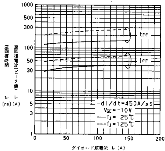
T_{rr}, I_{rr}-I_r 特性 T_{rr}, I_{rr}-I_r
