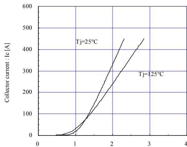
Collector current vs. Collector-Emitter voltage (typ.)
