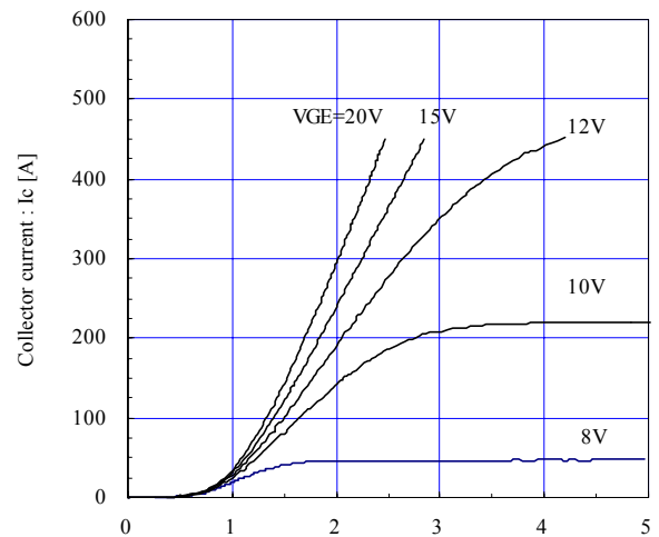
Collector current vs. Collector-Emitter voltage (typ.)
