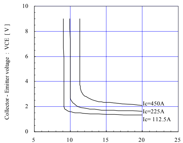
Collector-Emitter voltage vs. Gate-Emitter voltage (typ.)
