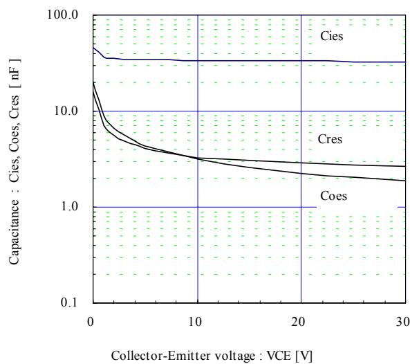
Capacitance vs. Collector-Emittter voltage (typ.)
