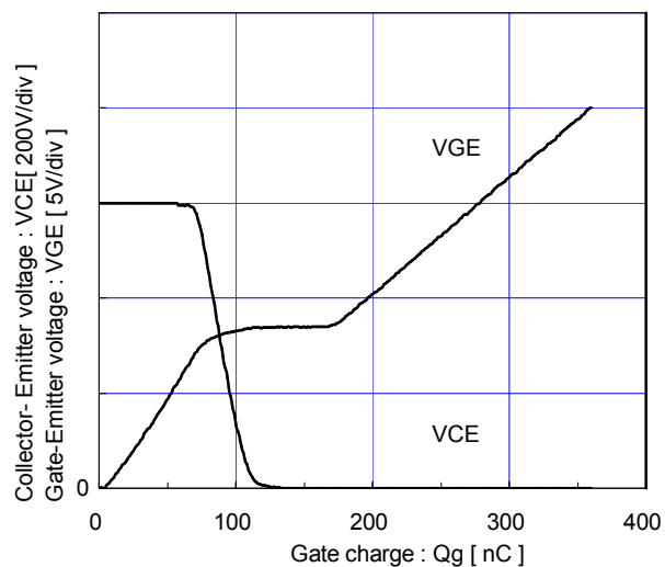
Dynamic Gate charge (typ.) Vcc=600V, Ic=75A, Tj=25°C
