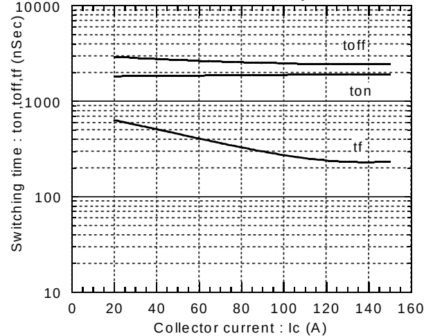
Switching time vs. Collector current Edc=600V,Vcc=15V,Tj=125°C
