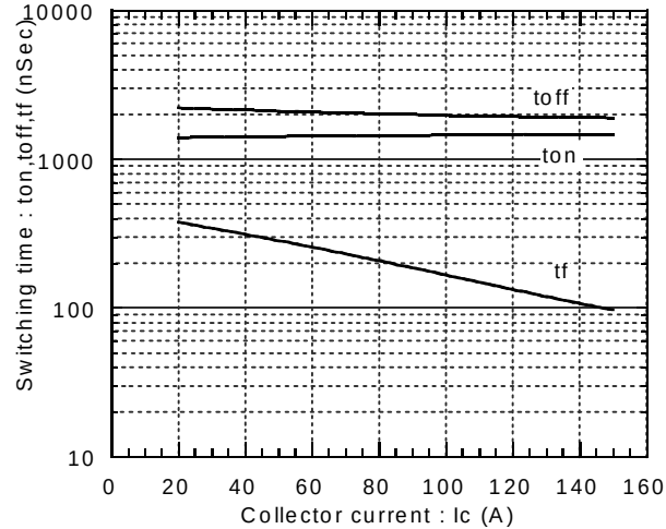
Switching time vs. Collector current Edc=600V,Vcc=15V,Tj=25°C
