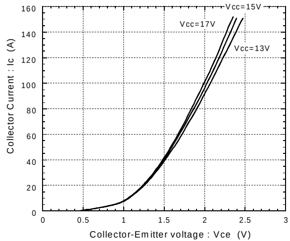
Collector current vs. Collector-Emitter voltage Tj=25°C
