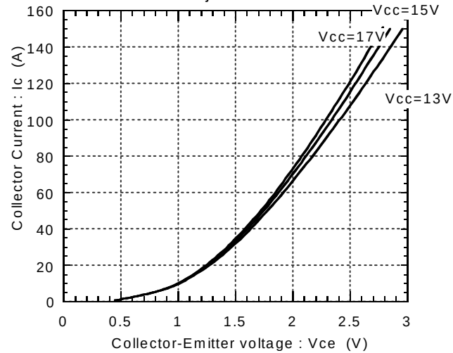
Collector current vs. Collector-Emitter voltage Tj=125°C
