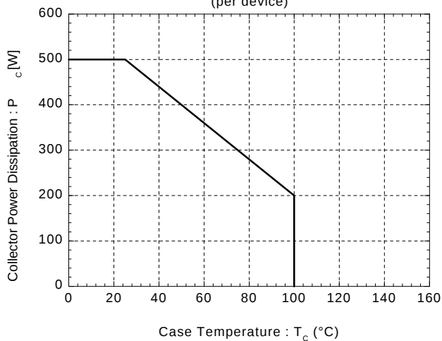
Power Derating For IGBT
