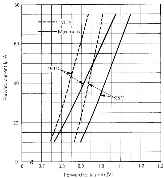
Forward Characteristics
