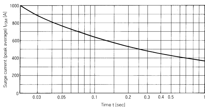
Surge Current
