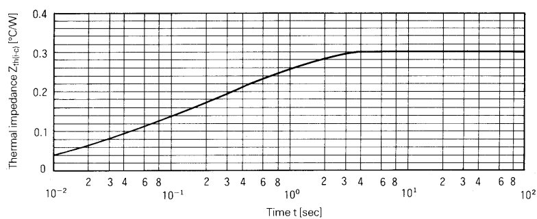
Transient Thermal Impedance
