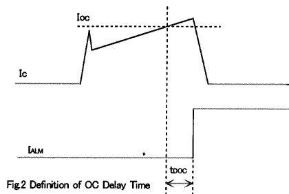
Fig.2 Definition of OC Delay Time
