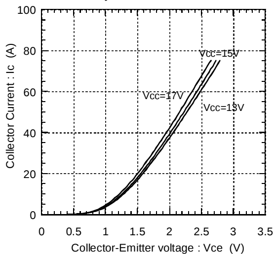
Collector current vs. Collector-Emmitter voltage (typ.) T_j=125^{\circ}\text{C} / Terminal
