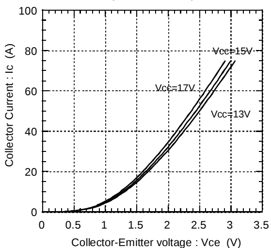
Collector current vs. Collector-Emmitter voltage (typ.) T_j=125^{\circ}\text{C} / Chip
