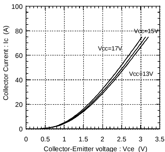
Collector current vs. Collector-Emmitter voltage (typ.) T_j=125^{\circ}\text{C} / Terminal
