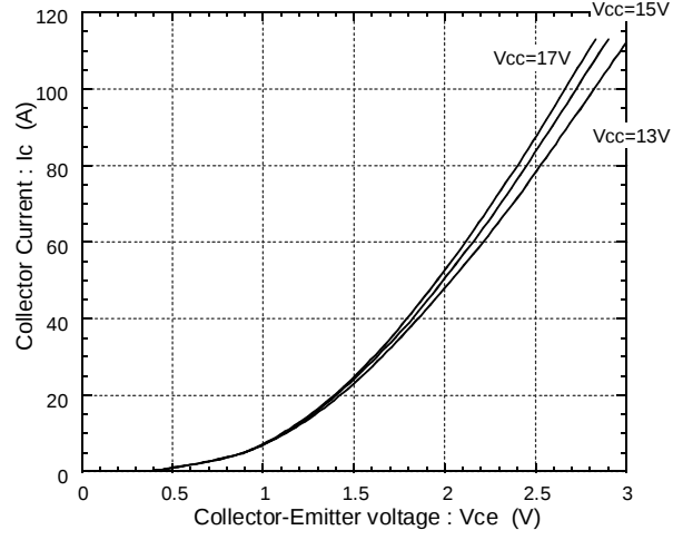
Collector current vs. Collector-Emitter voltage Tj=125°C
