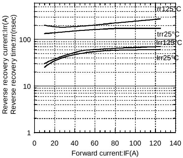
Reverse recovery characteristics (typ.) trr,Irr vs.IF
