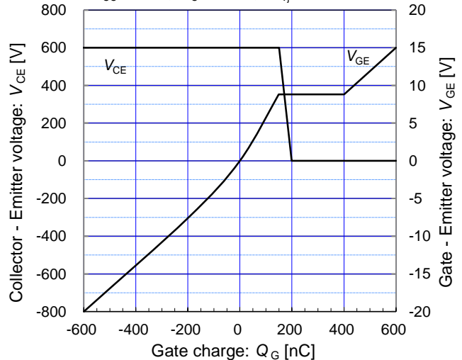
Dynamic Gate charge (typ.) V_{CC} = 600\text{V}, I_c = 150\text{A}, T_{vj} = 25^\circ\text{C}
