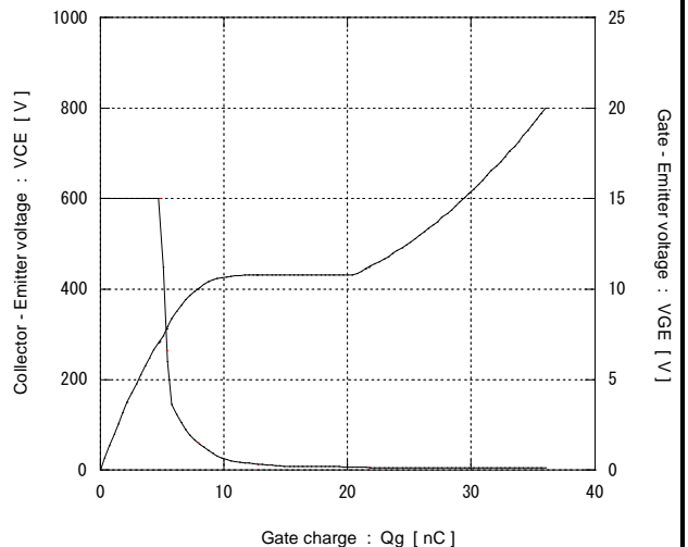
[ Brake ] Dynamic Gate charge (typ.) Vcc=600V, Ic=10A, Tj= 25°C
