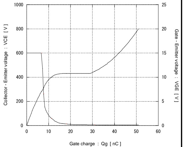
[ Inverter ] Dynamic Gate charge (typ.) Vcc = 600V, Ic = 15A, T j = 25°C
