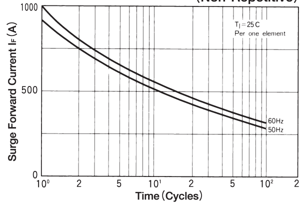
Cycle Surge Forward Current Rating
