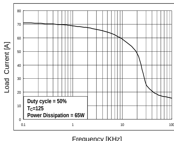
Fig 4. Load Current vs. Frequency
