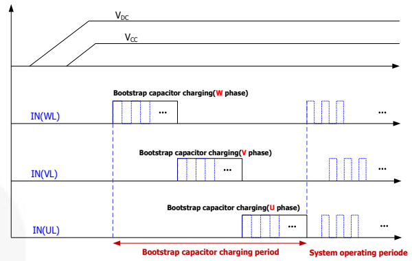
Figure 34. Recommended Initial Bootstrap Capacitors Charging Sequence
