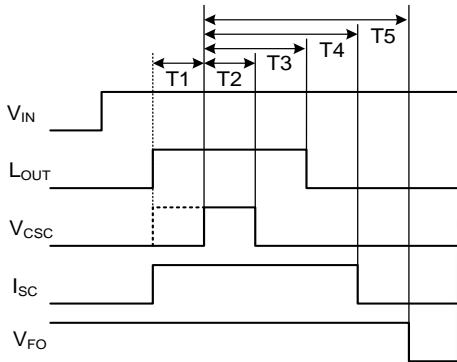
Figure 25. Timing Diagram
