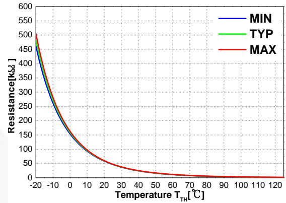
Figure 43. R-T Curve of NTC Thermistor
