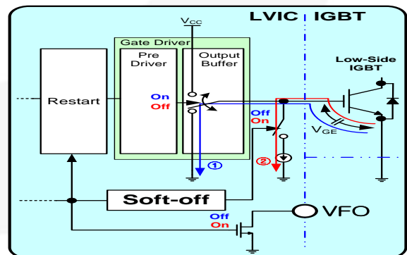
Figure 27. Operating Sequence of Soft Turn-Off
