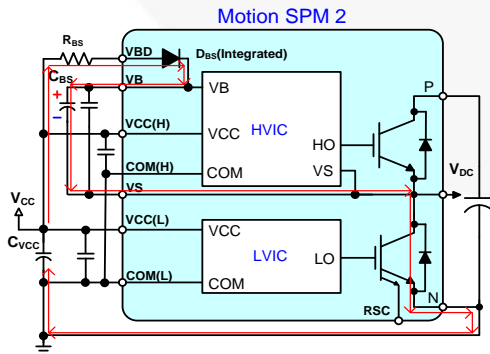
Figure 32. Current Path of Bootstrap Circuit for the Supply Voltage (V BS ) of a HVIC when Low-Side IGBT Turns On
