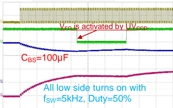
Figure 35. Initial Charging According to Bootstrap Capacitance and Charging Method (Ref. Condition: V_{CC}=15\text{ V}/300\text{ mA} , V_{CC} Capacitor= 220\text{ }\mu\text{F} , Bootstrap Capacitor= 100\text{ }\mu\text{F} , R_{BS}=20\text{ }\Omega )
