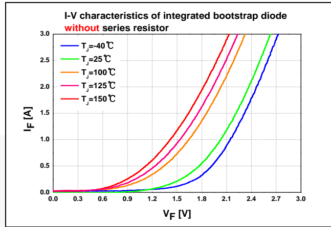
Figure 38. I-V Characteristics of Integrated Bootstrap Diode Series without Series Resistor
