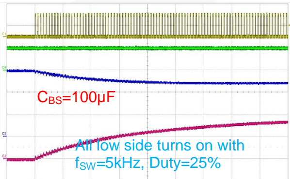
Figure 35. Initial Charging According to Bootstrap Capacitance and Charging Method (Ref. Condition: V_{CC}=15\text{ V}/300\text{ mA} , V_{CC} Capacitor= 220\text{ }\mu\text{F} , Bootstrap Capacitor= 100\text{ }\mu\text{F} , R_{BS}=20\text{ }\Omega )
