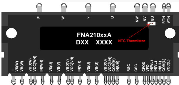
Figure 42. Location of NTC Thermistor in 1200-V Motion SPM 2
