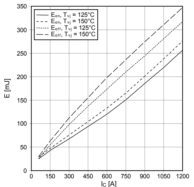
Schaltverluste IGBT-Wechselr. (typisch) switching losses IGBT-inverter (typical) E_{on} = f(I_C) , E_{off} = f(I_C) V_{GE} = \pm 15\text{ V} , R_{Gon} = 1.2\ \Omega , R_{Goff} = 1.2\ \Omega , V_{CE} = 900\text{ V}
