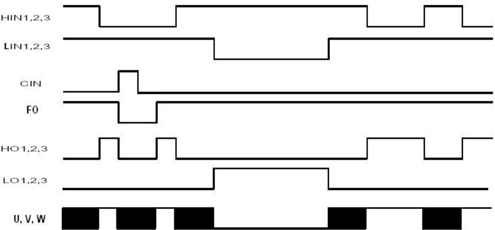
Figure 7. Input/Output Timing Diagram
