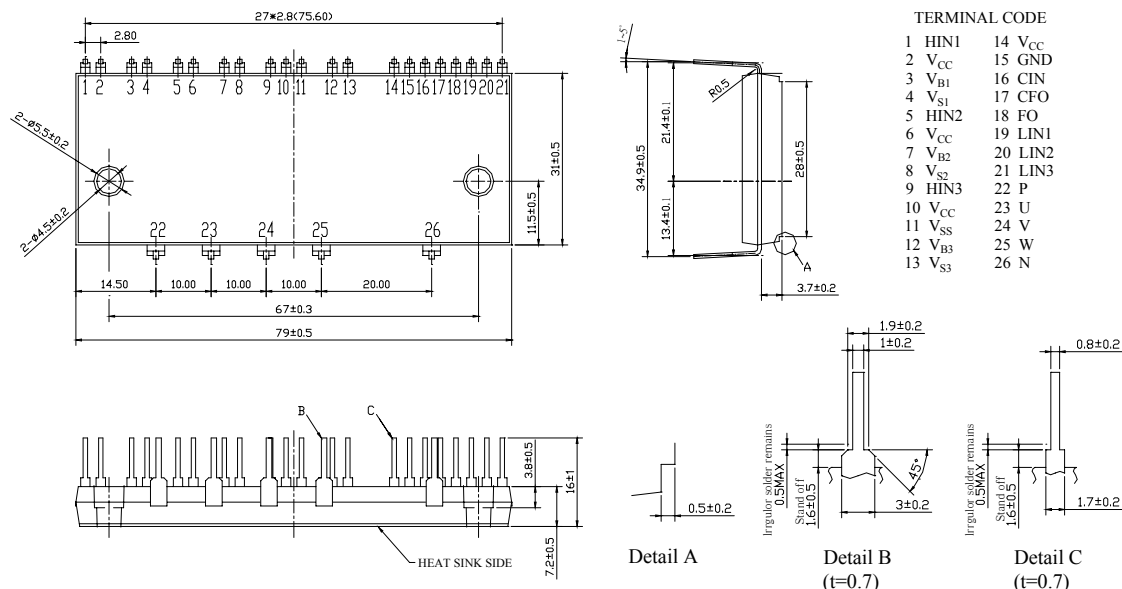
Figure 1. Package Outlines
