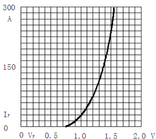
Fig1. Forward Characteristics
