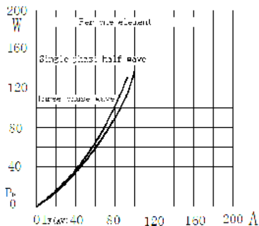
Fig2. Power dissipation
