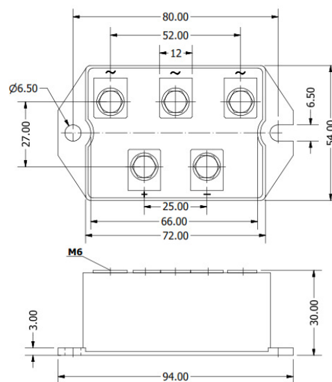
Package Type S
