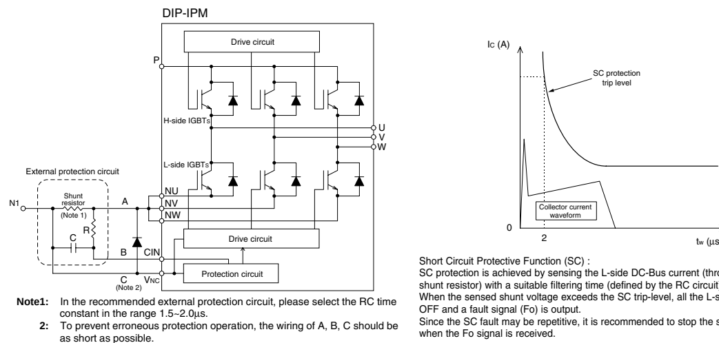
Fig. 3 EXTERNAL PART OF THE DIP-IPM PROTECTION CIRCUIT
